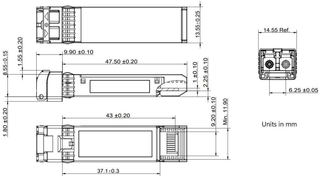
Figure2. Mechanical Outline
